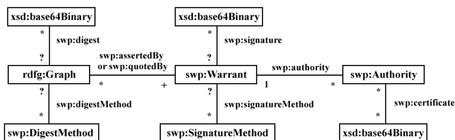
Figure 1.1: The Semantic Web Publishing Vocabulary (SWP).
