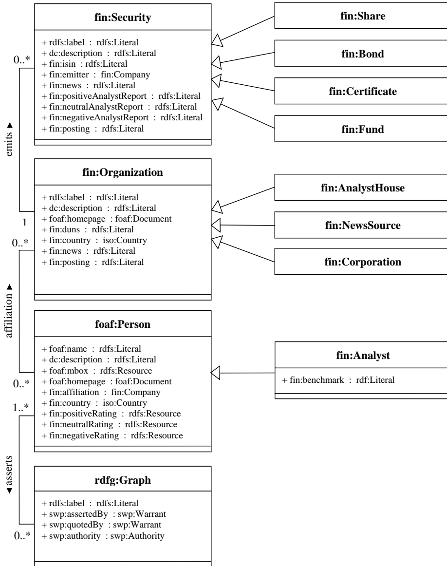
Figure 2.1: UML class diagram of the domain model.
